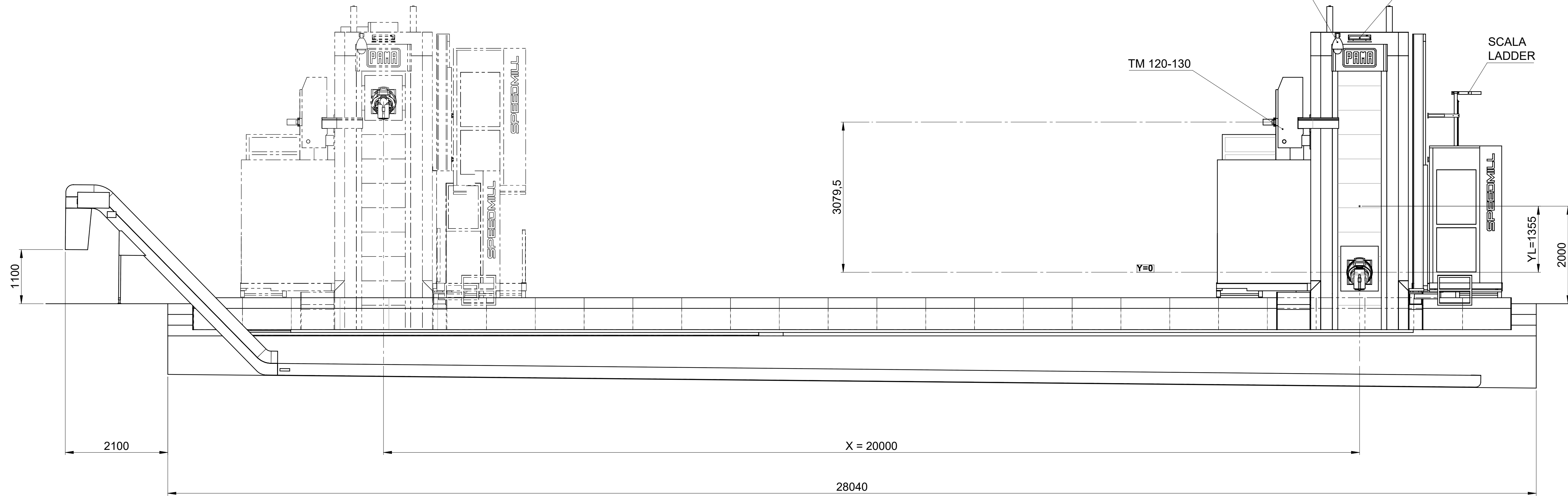
CORSE PEDANA OPERATORE OPERATOR PLATFORM'S STROKES
