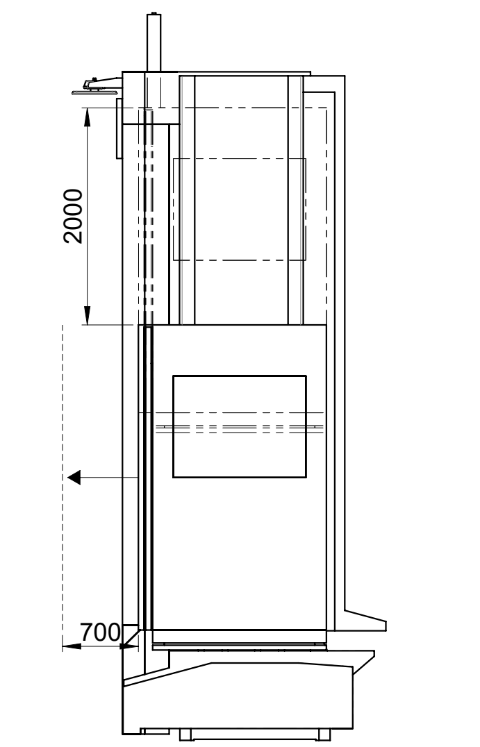
CORSE PEDANA OPERATORE OPERATOR PLATFORM'S STROKES
